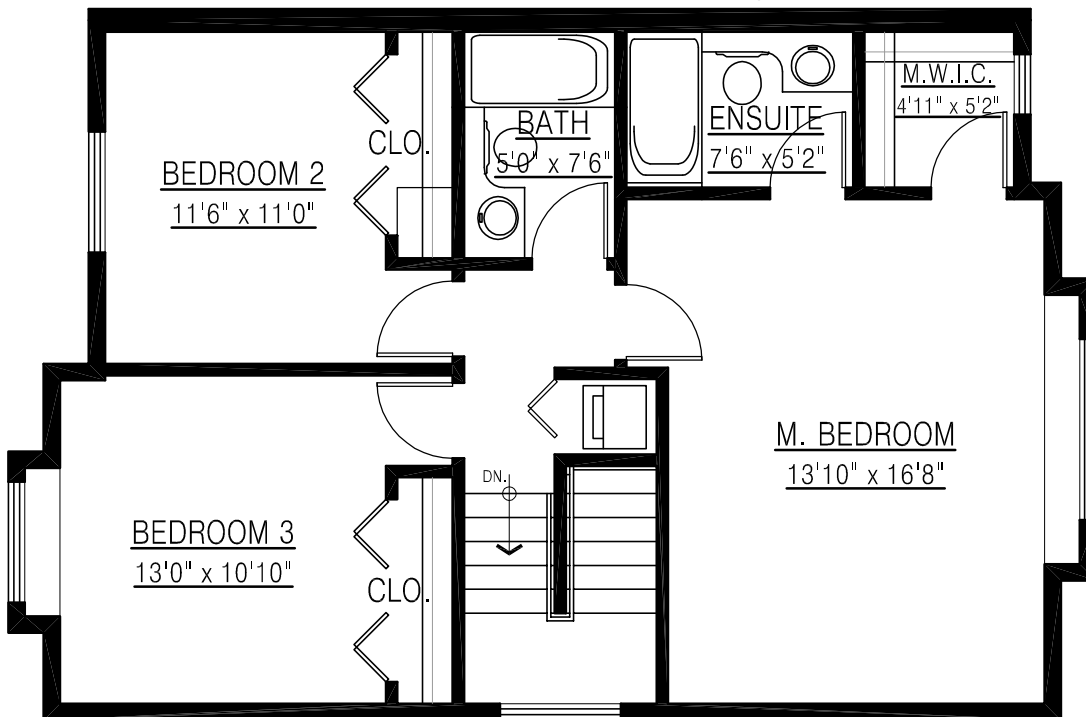
UPPER FLOOR PLAN-BUILDING B
