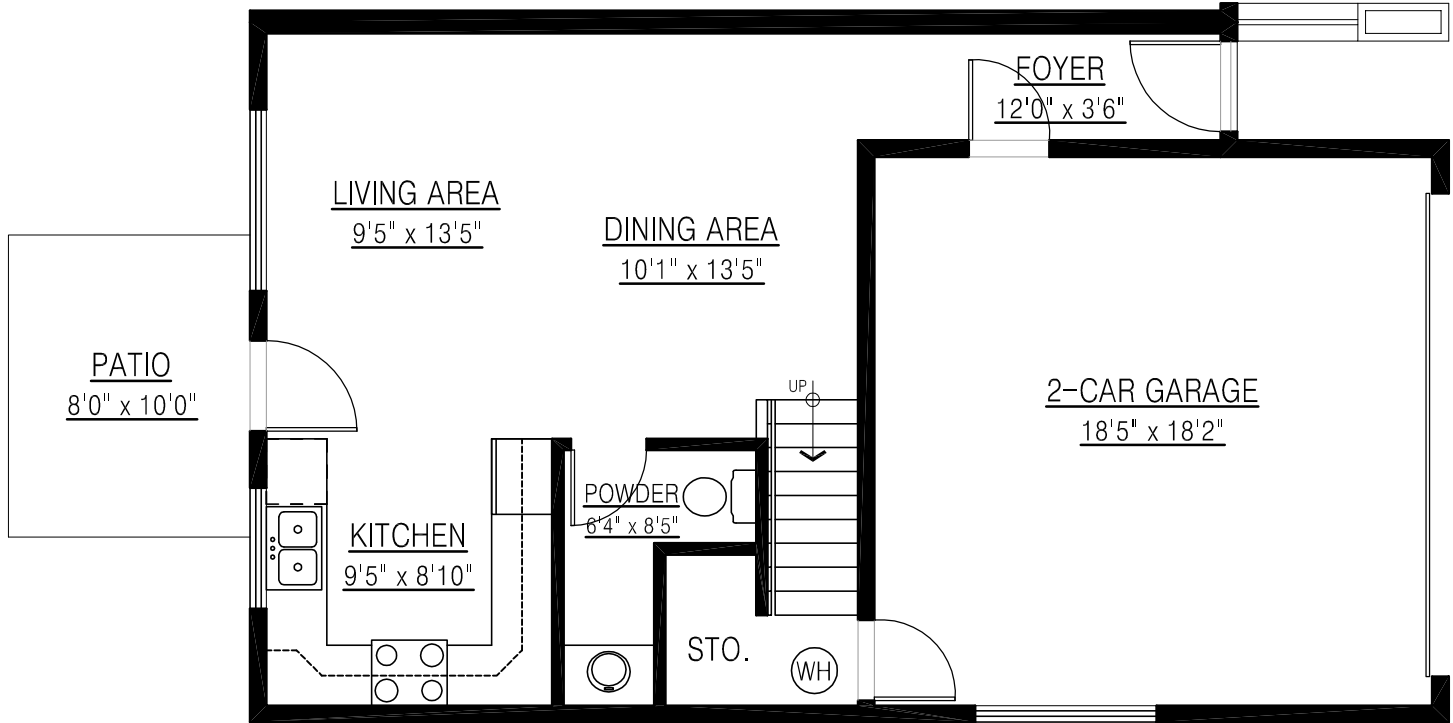
MAIN FLOOR PLAN-BUILDING B
