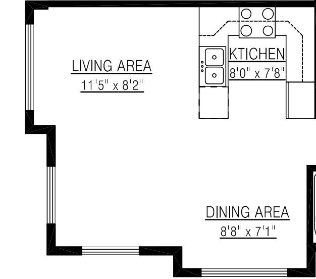
MAIN FLOOR PLAN-BUILDING A FLOOR AREA: 250 sq.ft.
