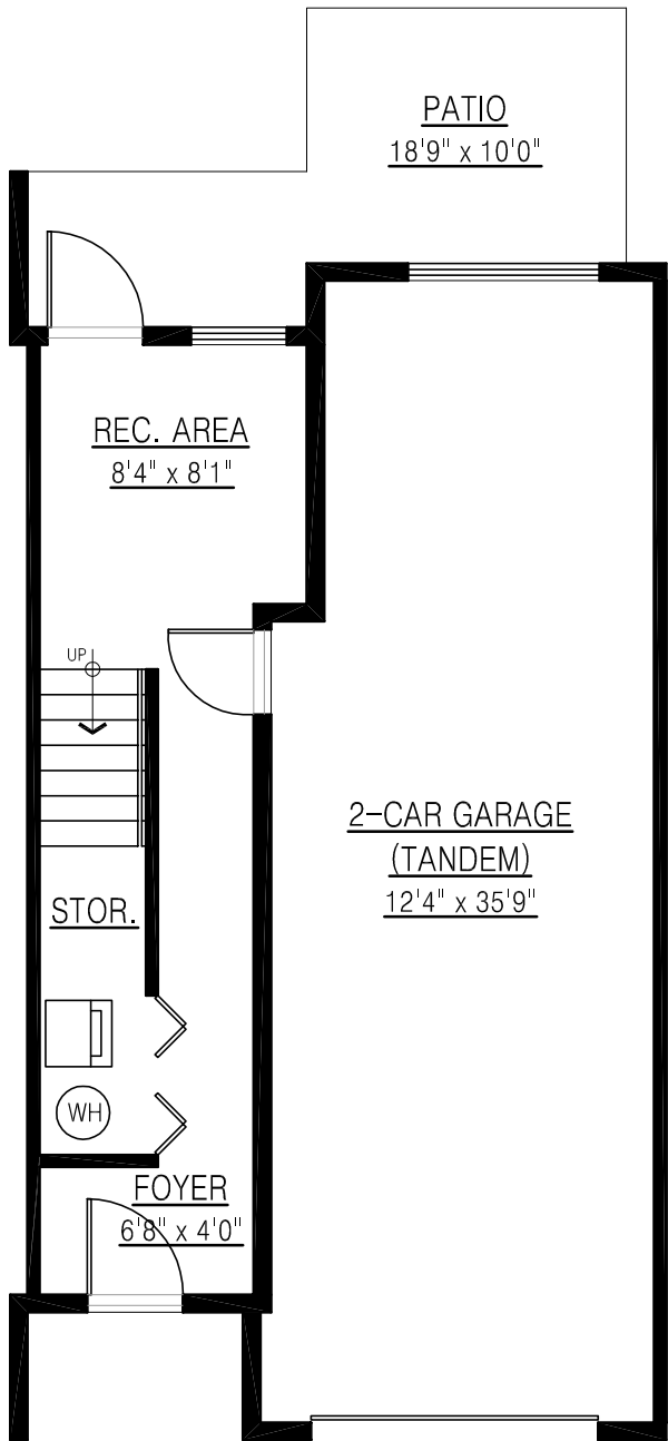
MAIN FLOOR PLAN-BUILDING A FLOOR AREA: 250 sq.ft.
