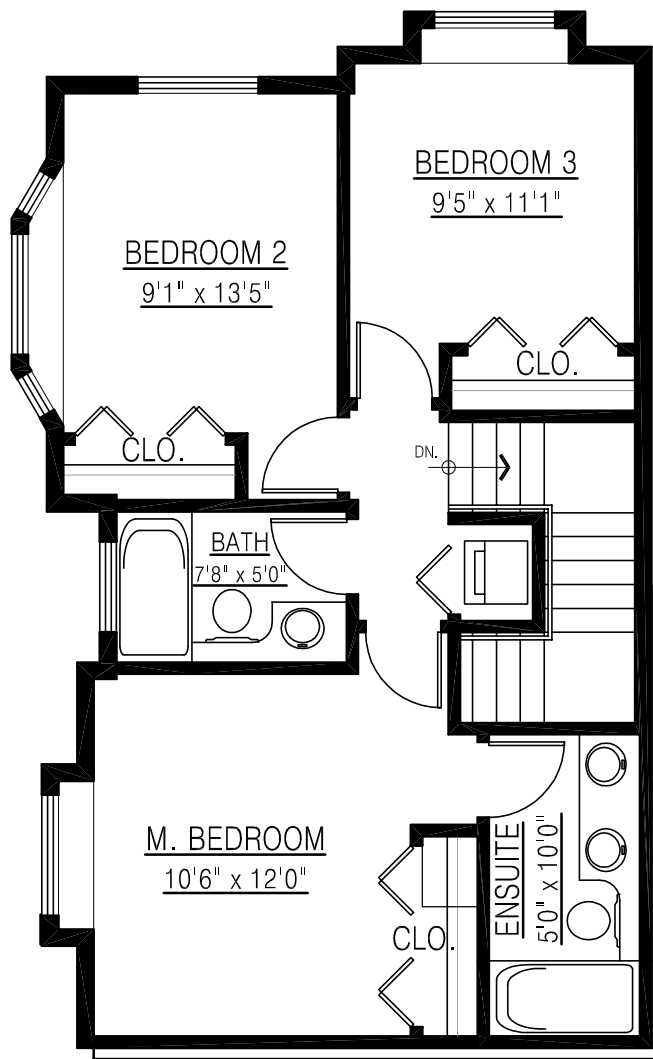
UPPER FLOOR PLAN-BUILDING A FLOOR AREA: 654 sq.ft.
